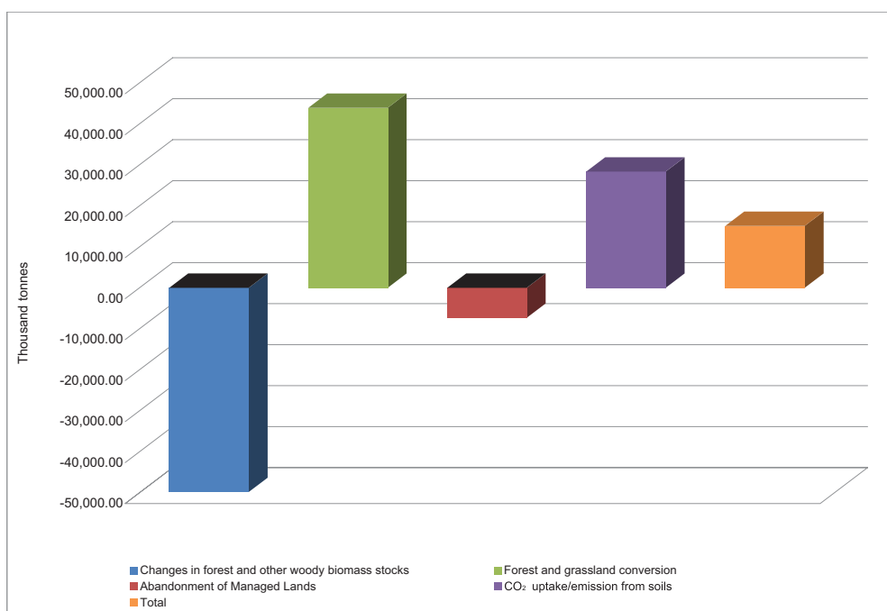
Figure 2.5. GHG emissions from LULUCF in 2000
