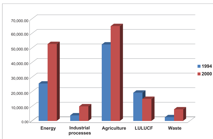
Figure 2.9. GHG emissions by sector, in 1994 and 2000
