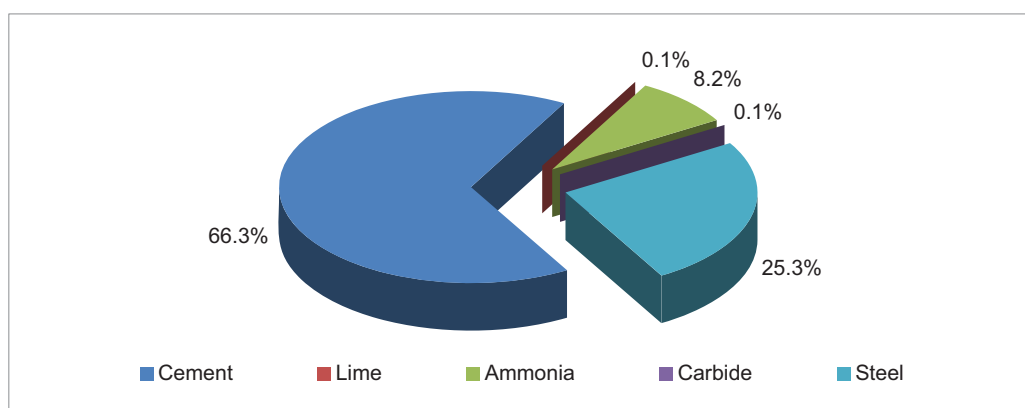
Figure 2.3. GHG emissions from industrial processes in 2000
