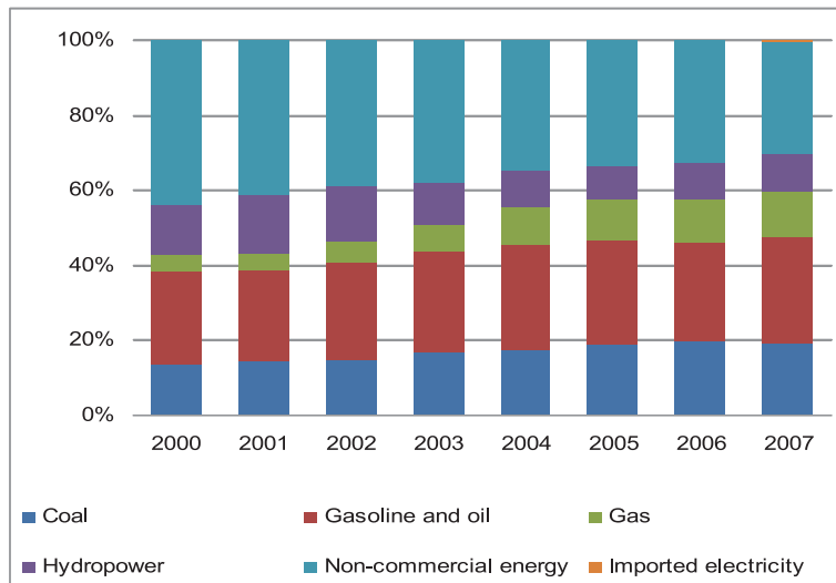
Figure 1.2. Structure of primary energy from 2000 to 2007
