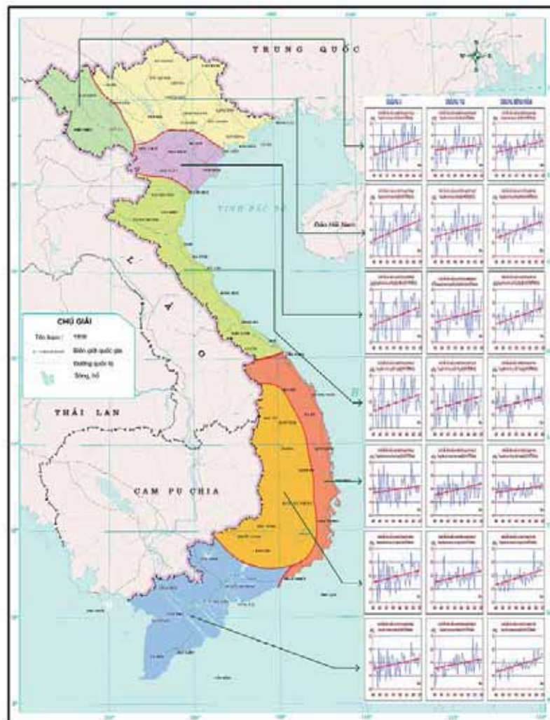
Figure 3.1. Temperature trends
