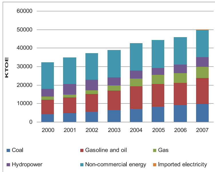
Figure 1.1. Primary energy consumption by type of energy
