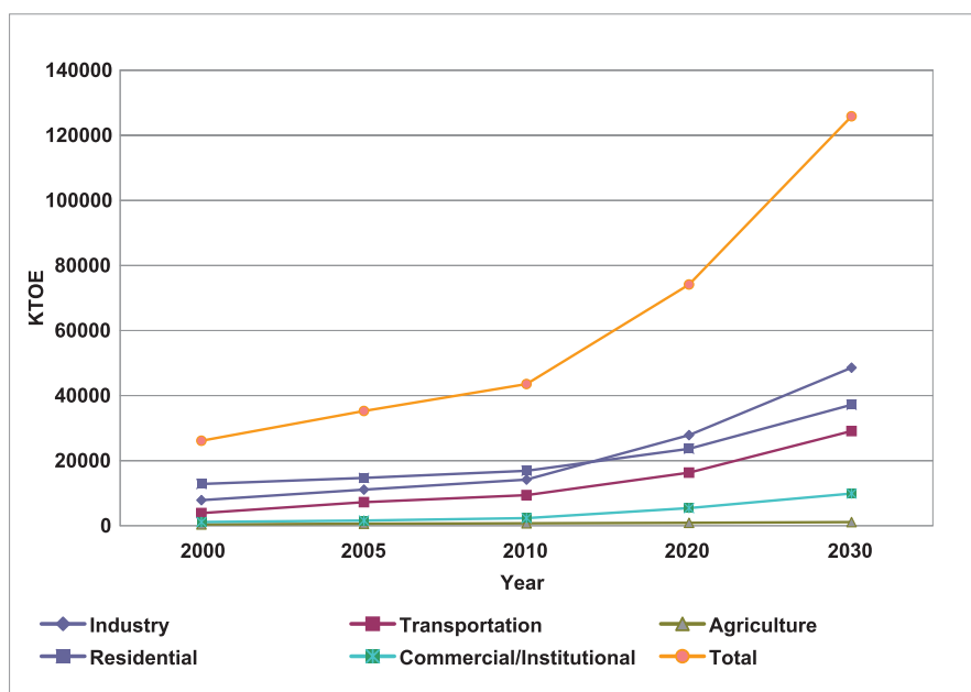
Figure 4.1. Energy demand projections by sector
