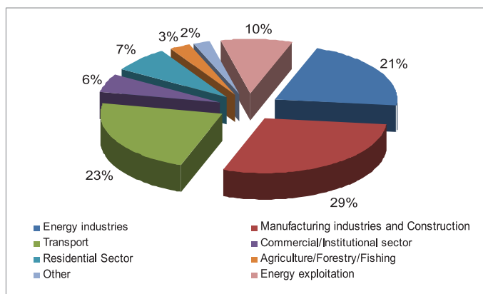
Figure 2.2. GHG emissions from energy
