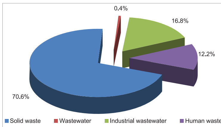
Figure 2.6. GHG emissions from waste in 2000
