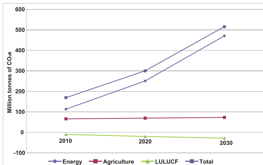
Figure 2.10. GHG emission projections 2010-2030
