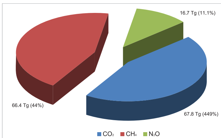
Figure 2.8. GHG emissions by gas in CO 2 e
