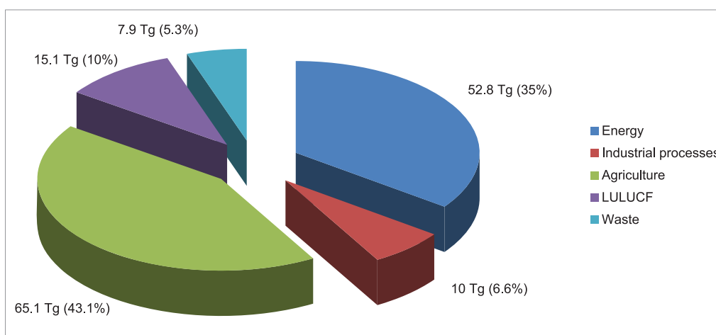
Figure 2.7. GHG emissions by sector in 2000 in CO 2 e
